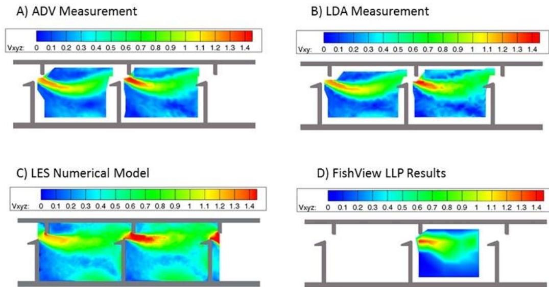
Fig. 3. Comparison of current velocity estimates between A) Acoustic Doppler Velocimetry, B) Laser Doppler Velocimetry, C) Large Eddy Simulation 3D model, and D) our BONUS FISHVIEW Lateral Line Probe. The simulation shows that our probe accurately estimates the real flow conditions in fishpasses.
